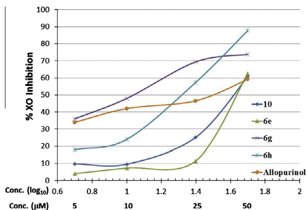
Fig. 5. Semilog plot of concentration vs % inhibition of xanthine oxidase (XO) enzyme. The IC 50 is identified from the midpoint (i.e., 50% inhibition) of the semilog plot.
