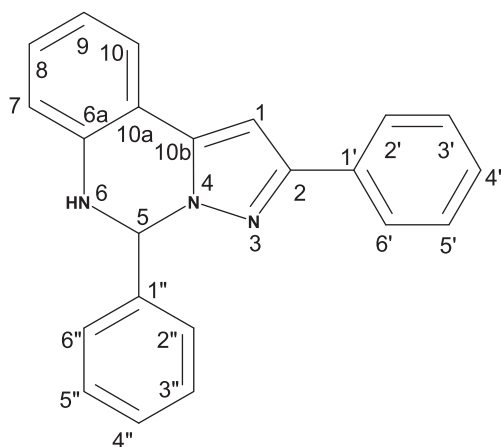
Fig. 3. Numbering to the target compounds 5 and 6 .
